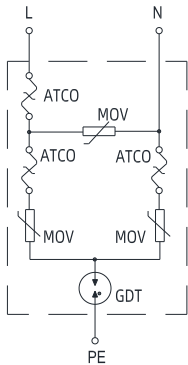
SD05CxxxGM Series FIGURE SD05C-2
