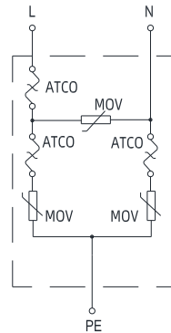
SD05CxxxNM Series FIGURE SD05C-4
