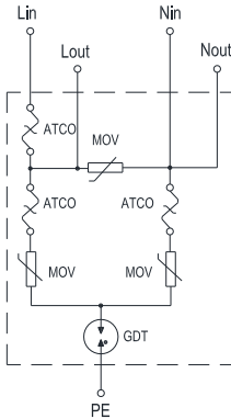
SD05CxxxGMT Series FIGURE SD05C-6
