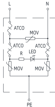
SD05CxxxLM Series FIGURE SD05C-3
