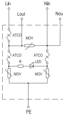
SD05CxxxLMT Series FIGURE SD05C-7
