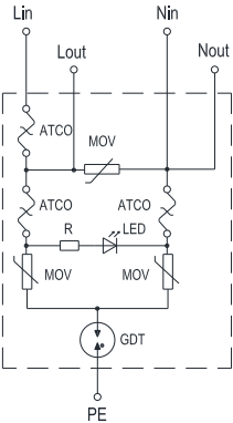
SD05CxxxAMT Series FIGURE SD05C-5
