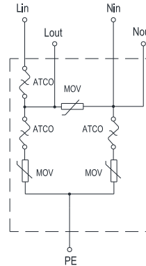
SD05CxxxNMT Series FIGURE SD05C-8
